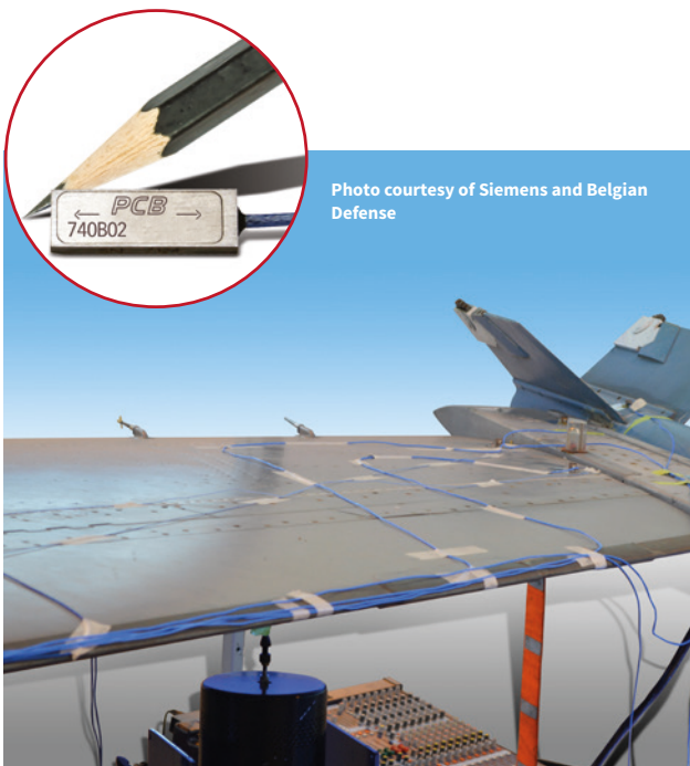
Model 740B02 strain sensors installed on a composite wing structure.
