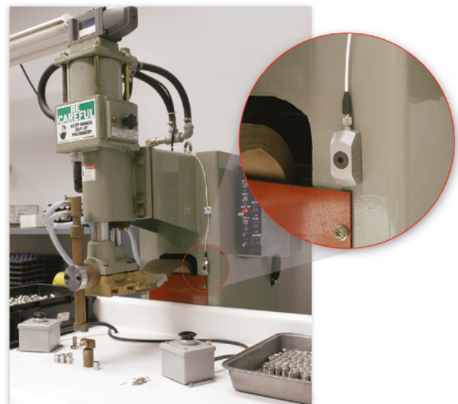
The RHM240 series strain sensor monitors press-fit forces to ensure quality end products.
